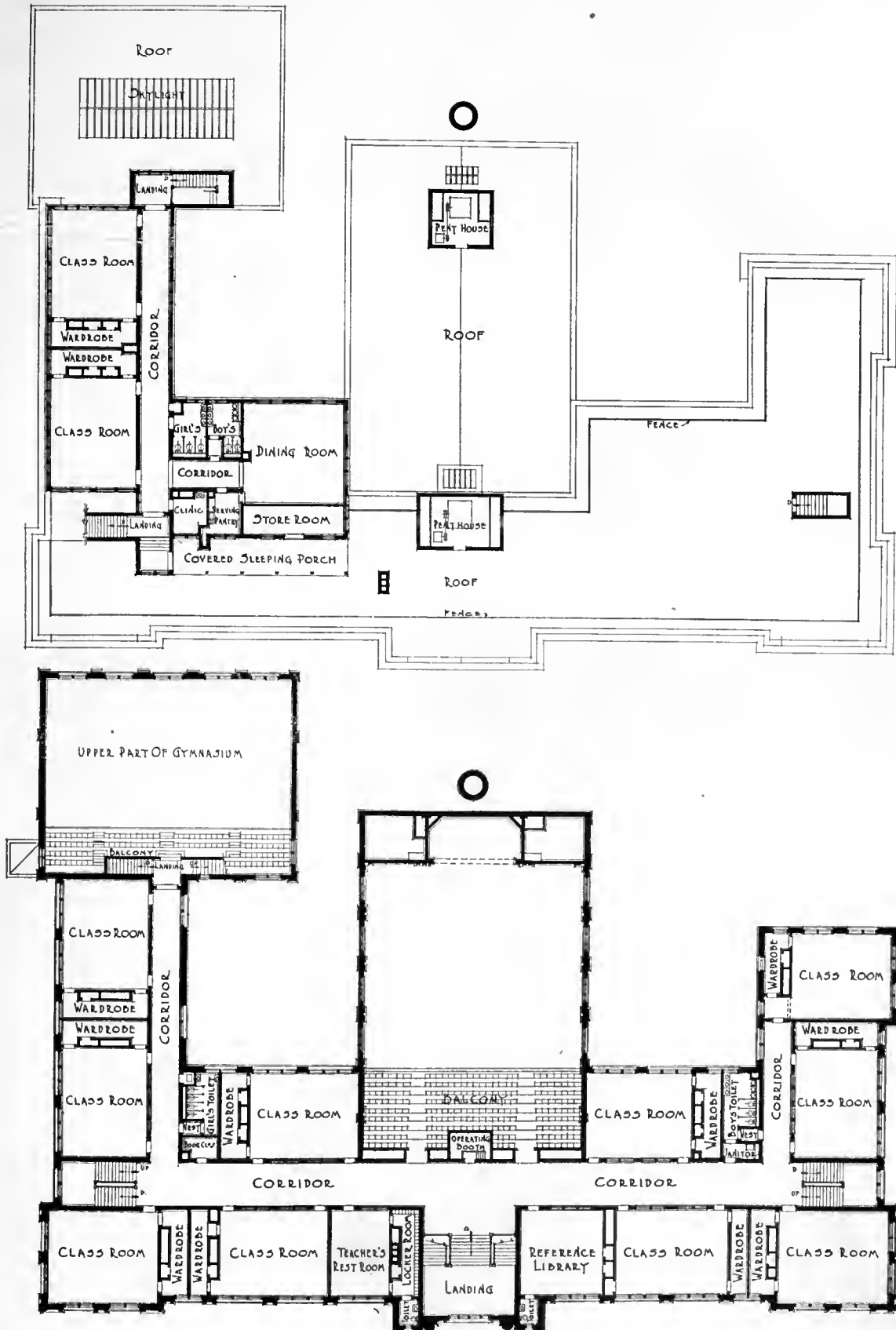
SECOND FLOOR AND ROOF PLANS DELAWARE SCHOOL, SYRACUSE, NEW YORK JAMES A. RANDALL, ARCHITECT
